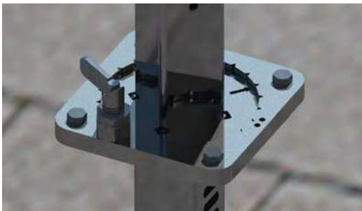
Fully Adjustable Solar Panel Orientation
